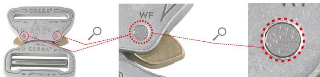
Fig. 2: Wrong: The rivet shows no imprint in the shape of a ring
