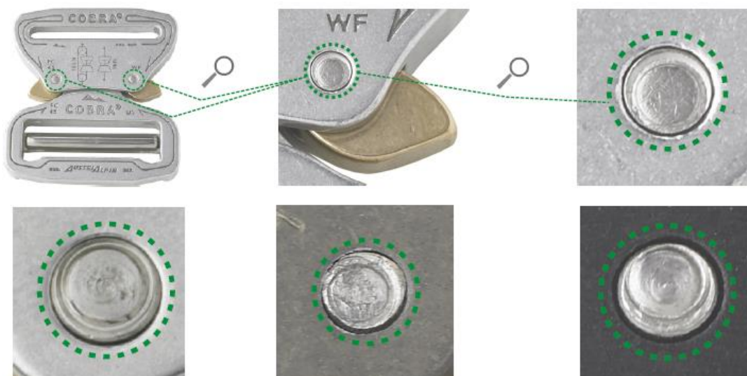
Fig. 1: Correct: The rivet shows an imprint in the shape of a ring on the front- and back side
